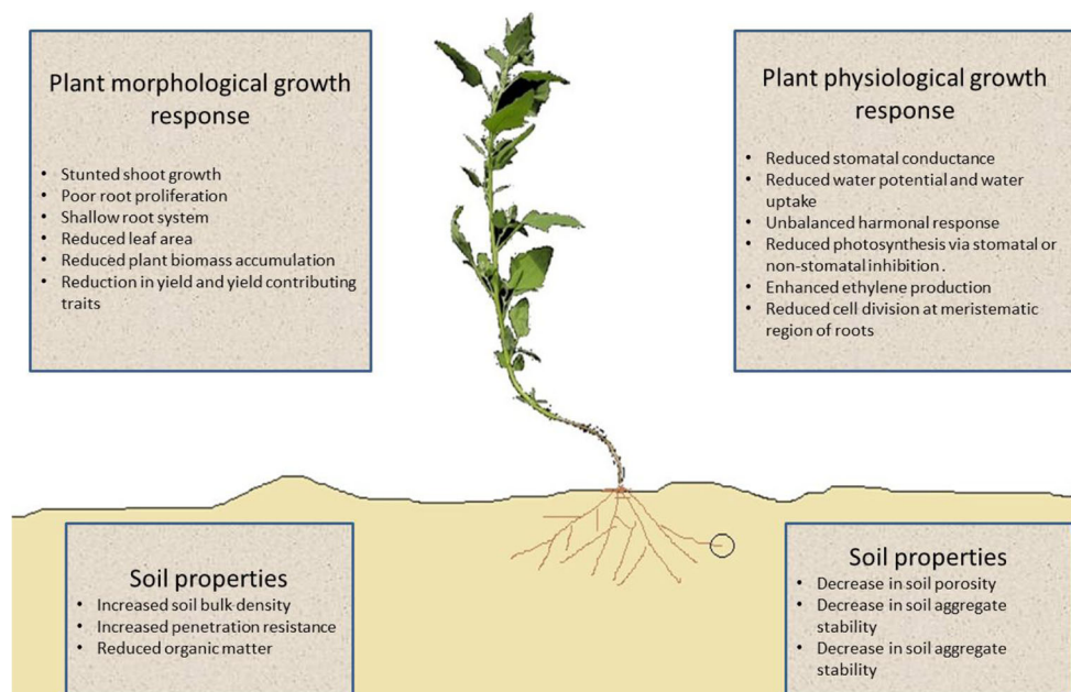
Fig. 2 Summary of the knowledge of the effects of soil compaction on soil plant morphological and physiological growth and soil properties
